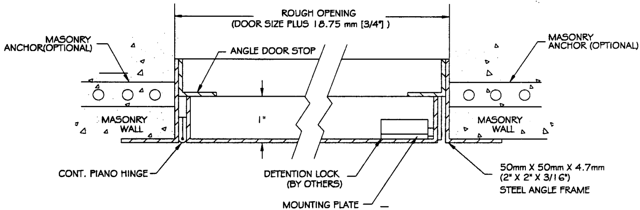
A CUT-THRU SECTION A NOT TO SCALE
