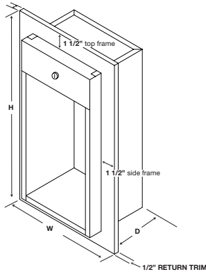
SEMI-RECESSED 999-SR (10 LB) ROUGH OPENING DIMENSIONS
