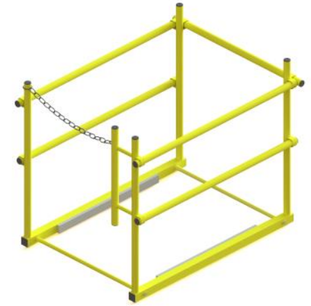
SHWC-3636 SHOWN WITH STANDARD GRAB BAR (Standard with 36" and Greater Egress)
