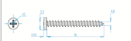
(DIN 7505B) SCREW D-05x50 ZB
