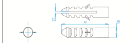
NYLON PLUG D8
