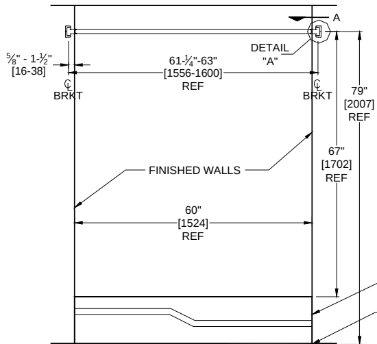
INSTALLATION TYPE A - FACE WALLS
