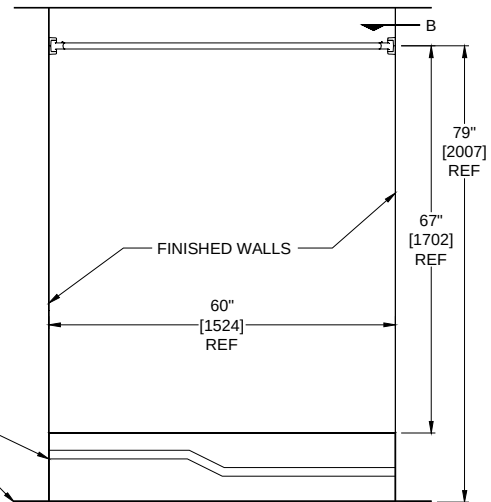
INSTALLATION TYPE B - OPPOSITE WALLS
