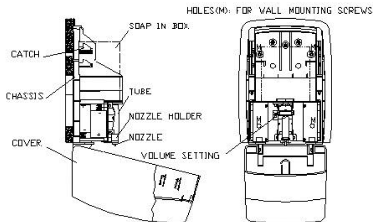
FIG. 3 PARTS DIAGRAM
