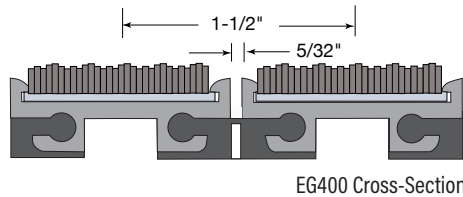
EG400 Cross-Section
