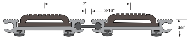
EM701 Cross-Section
